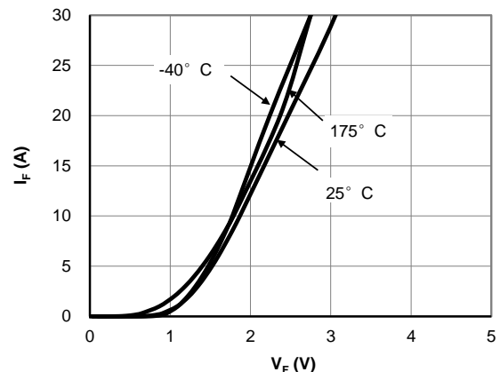
Figure 4: Diode Characteristic
